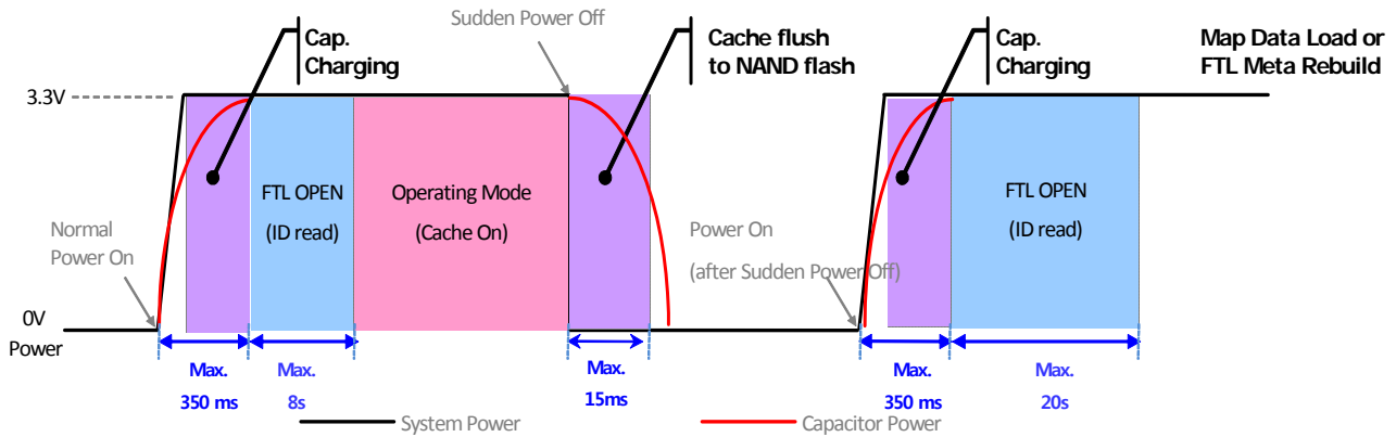
Figure 2. Sudden Power on-off operation
